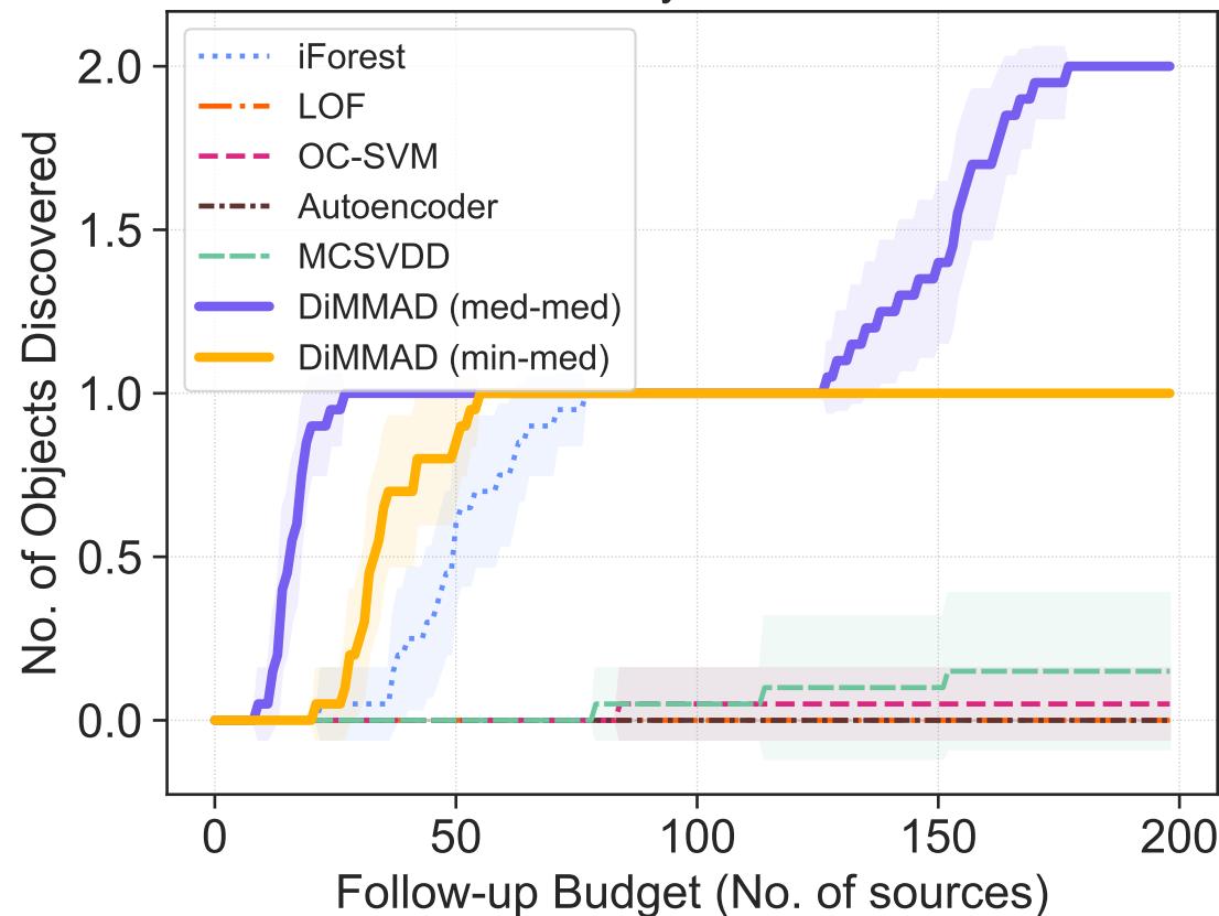
Anomaly: SL-SNIc
